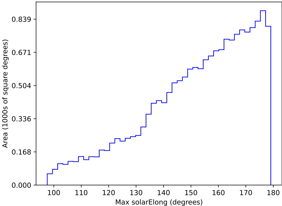
roll_pause_mjdp120_v3.4_10yrs WFD u band: Max solarElong
