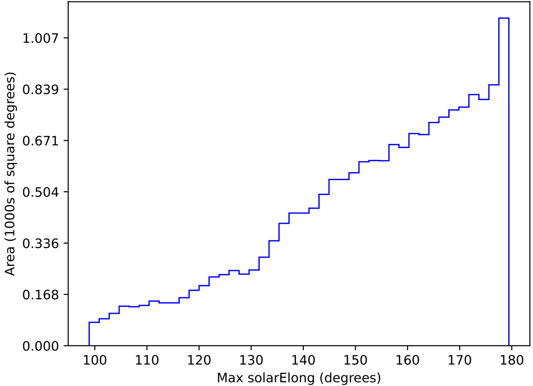
roll_pause_mjdp120_v3.4_10yrs WFD i band: Max solarElong
