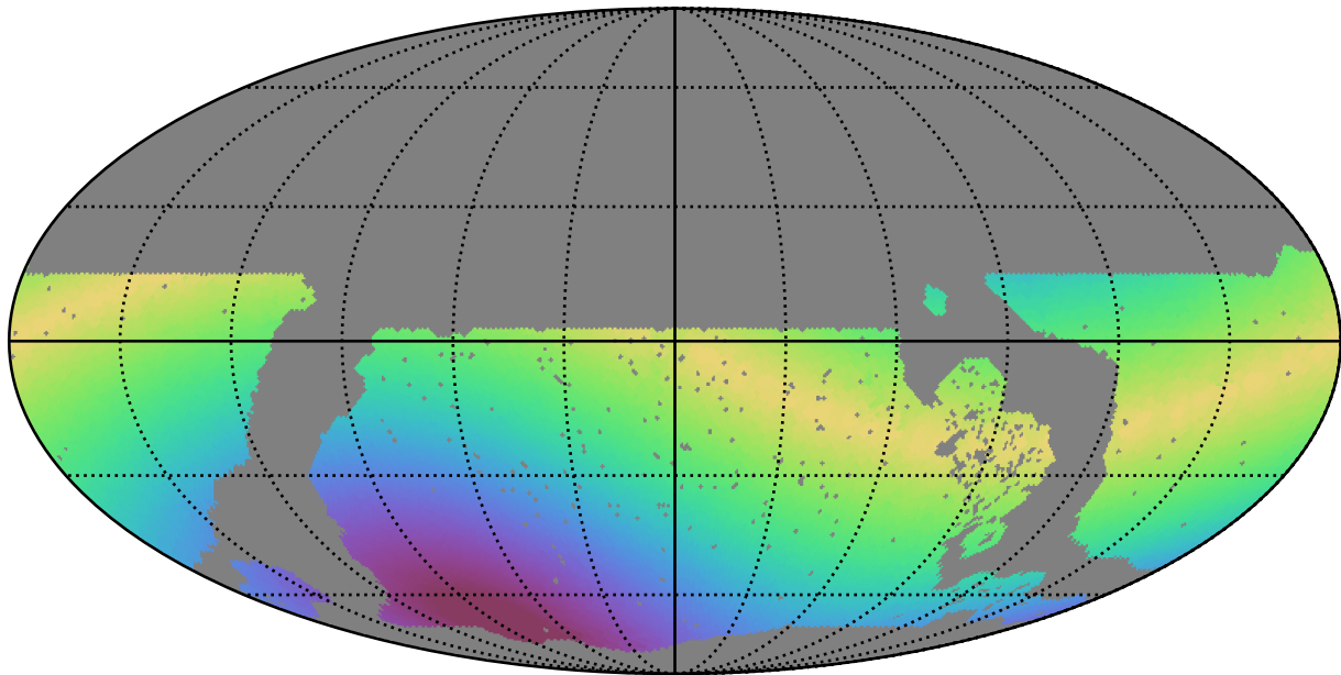
roll_pause_mjdp120_v3.4_10yrs WFD g band: Max solarElong
