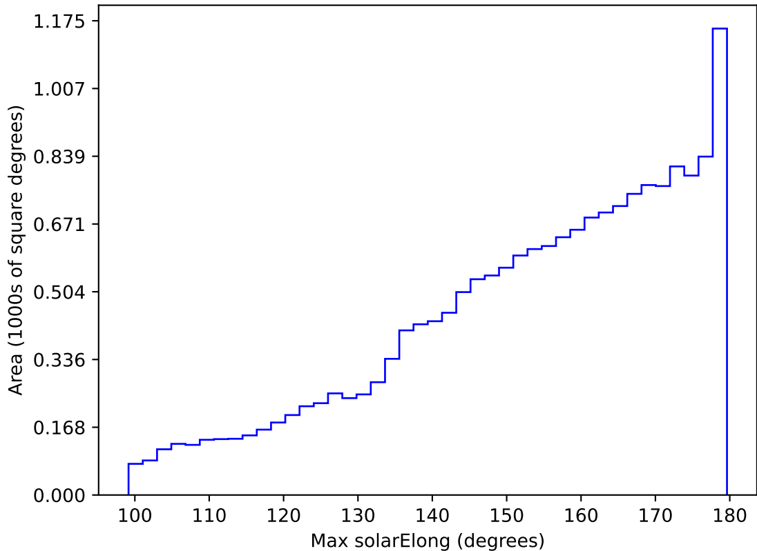
roll_pause_mjdp120_v3.4_10yrs WFD all bands: Max solarElong
