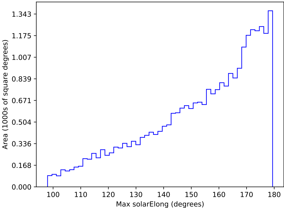
roll_pause_mjdp120_v3.4_10yrs All sky z band: Max solarElong
