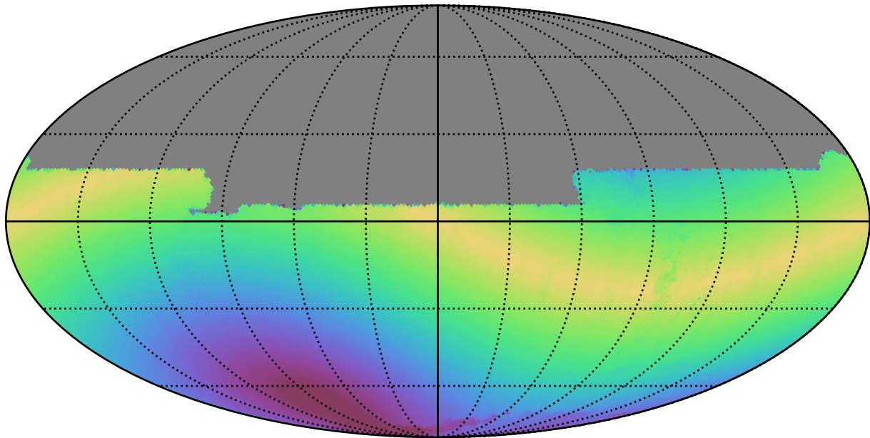
roll_pause_mjdp120_v3.4_10yrs All sky y band: Max solarElong
