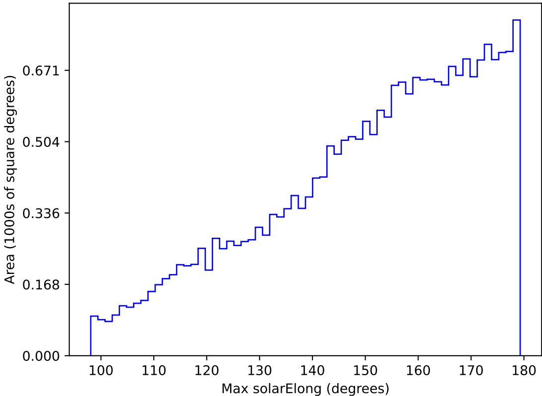
roll_pause_mjdp120_v3.4_10yrs All sky y band: Max solarElong
