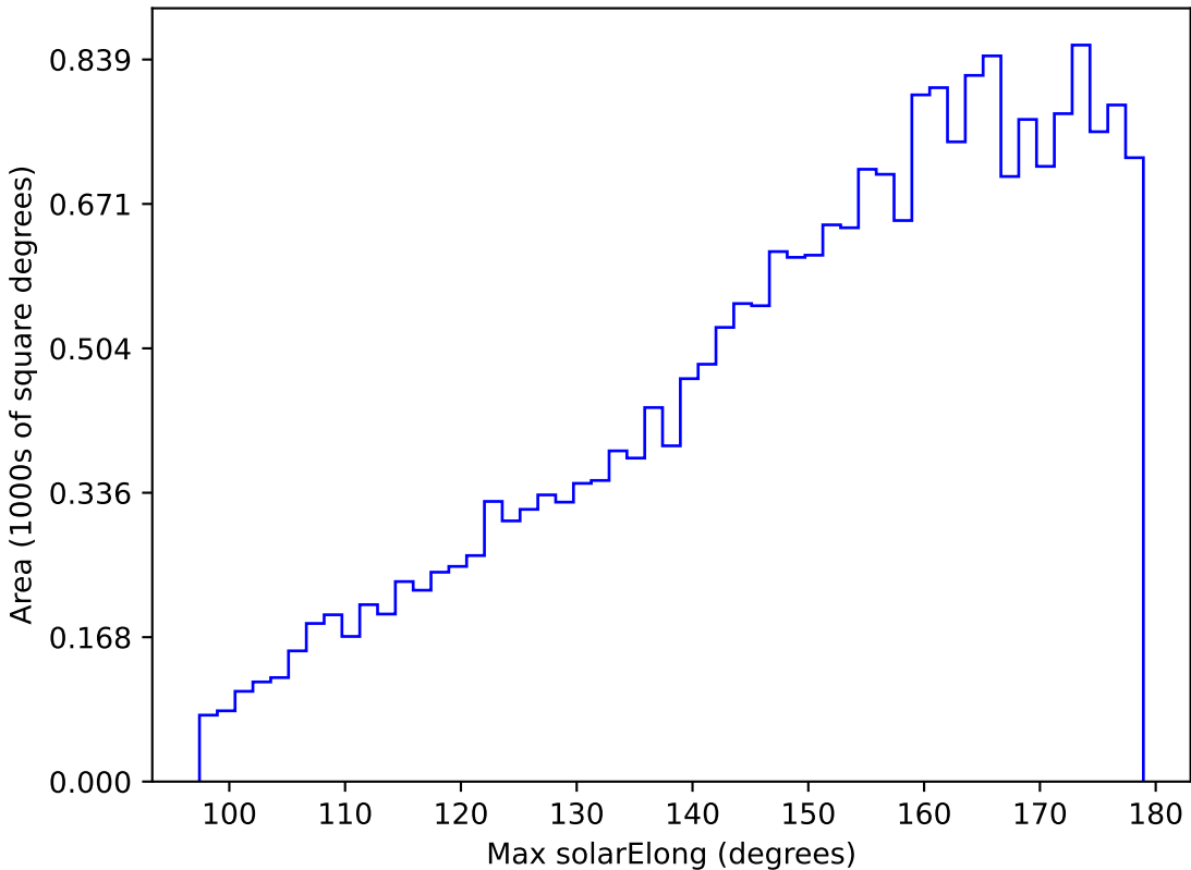
roll_pause_mjdp120_v3.4_10yrs All sky u band: Max solarElong
