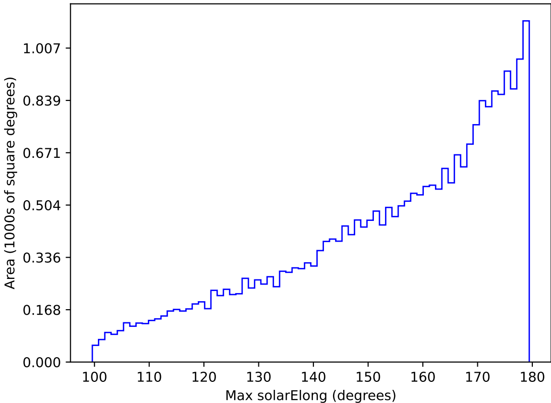
roll_pause_mjdp120_v3.4_10yrs All sky r band: Max solarElong
