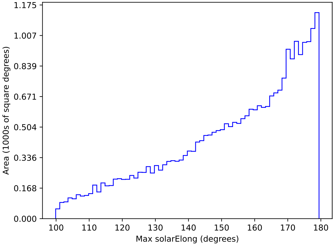
roll_pause_mjdp120_v3.4_10yrs All sky i band: Max solarElong
