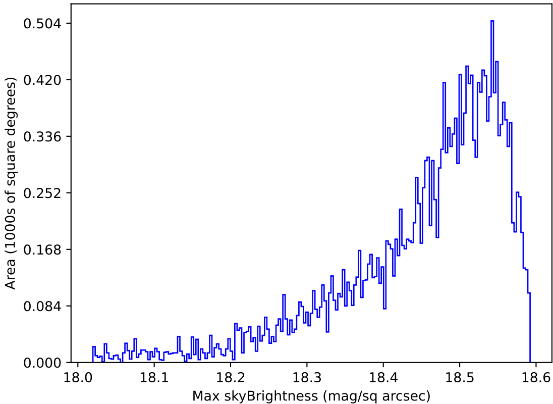
roll_pause_mjdp120_v3.4_10yrs Yr 1 y band: Max skyBrightness
