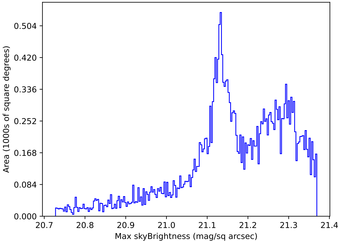
roll_pause_mjdp120_v3.4_10yrs Yr 1 r band: Max skyBrightness
