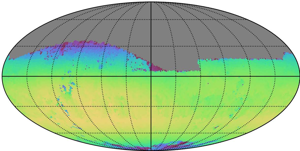
roll_pause_mjdp120_v3.4_10yrs Yr 1 i band: Max skyBrightness
