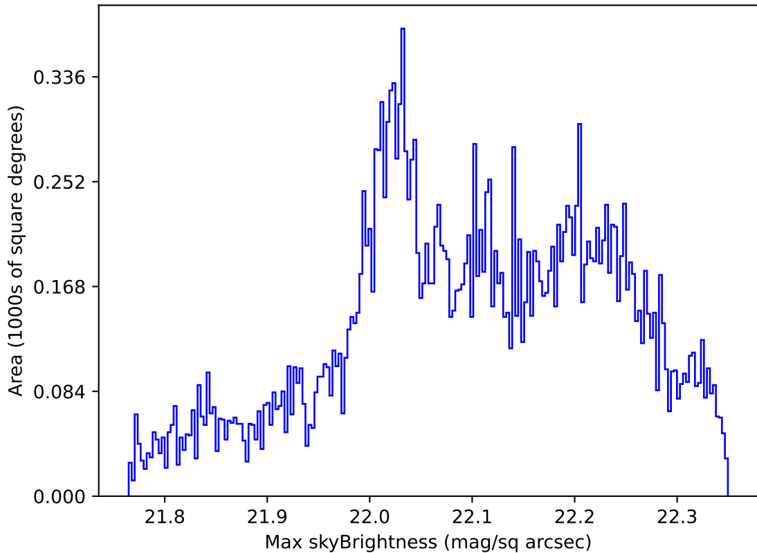
roll_pause_mjdp120_v3.4_10yrs Yr 1 g band: Max skyBrightness
