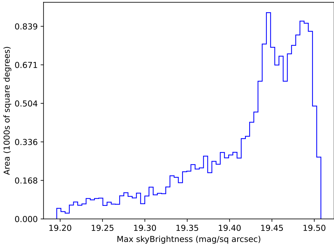
roll_pause_mjdp120_v3.4_10yrs WFD z band: Max skyBrightness
