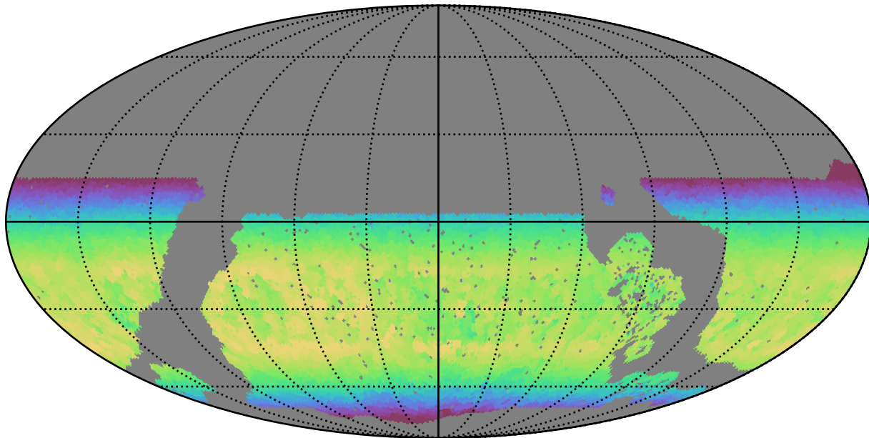
roll_pause_mjdp120_v3.4_10yrs WFD y band: Max skyBrightness
