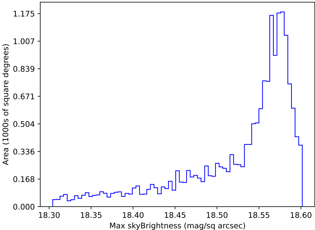
roll_pause_mjdp120_v3.4_10yrs WFD y band: Max skyBrightness
