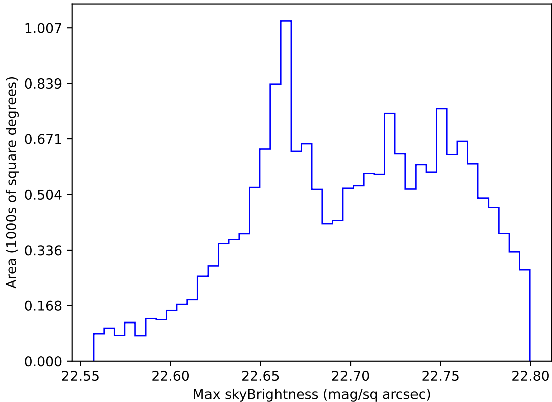
roll_pause_mjdp120_v3.4_10yrs WFD u band: Max skyBrightness
