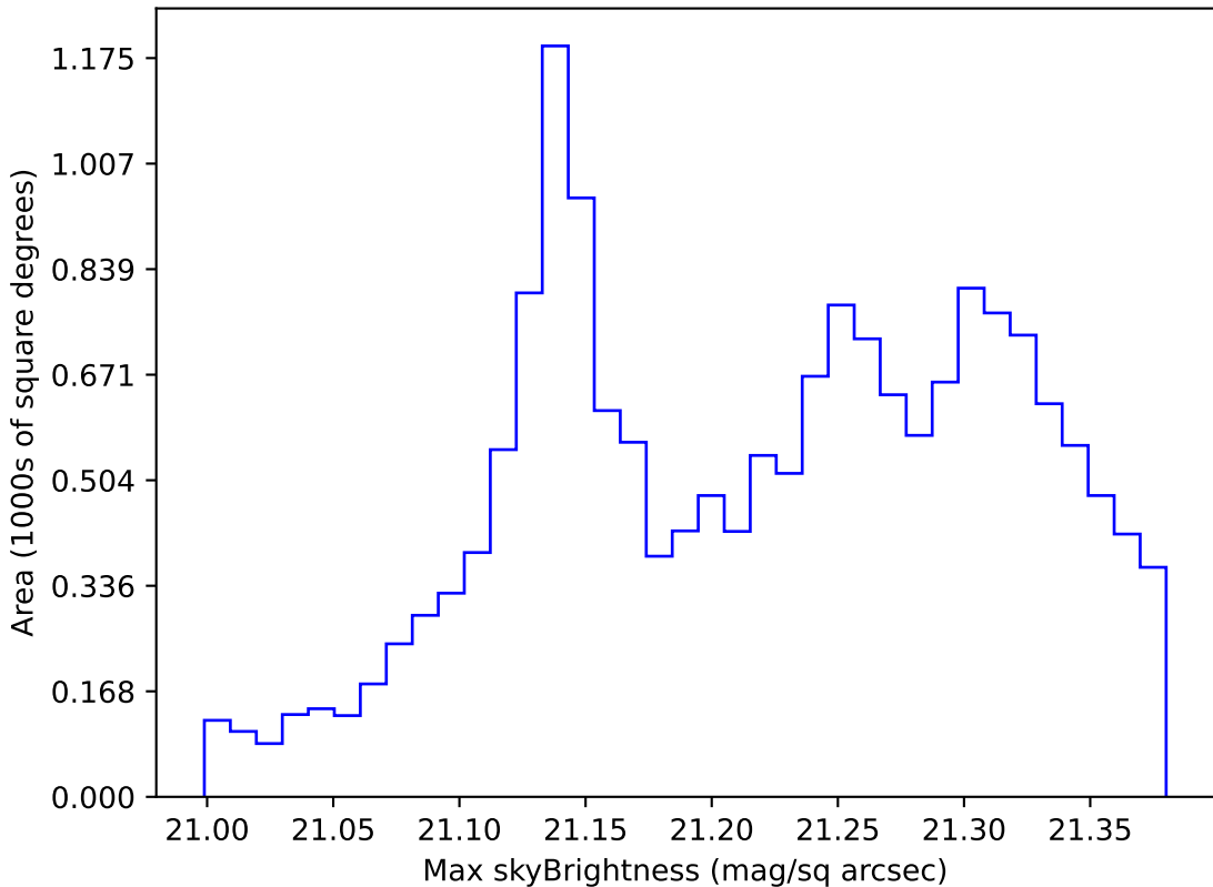
roll_pause_mjdp120_v3.4_10yrs WFD r band: Max skyBrightness
