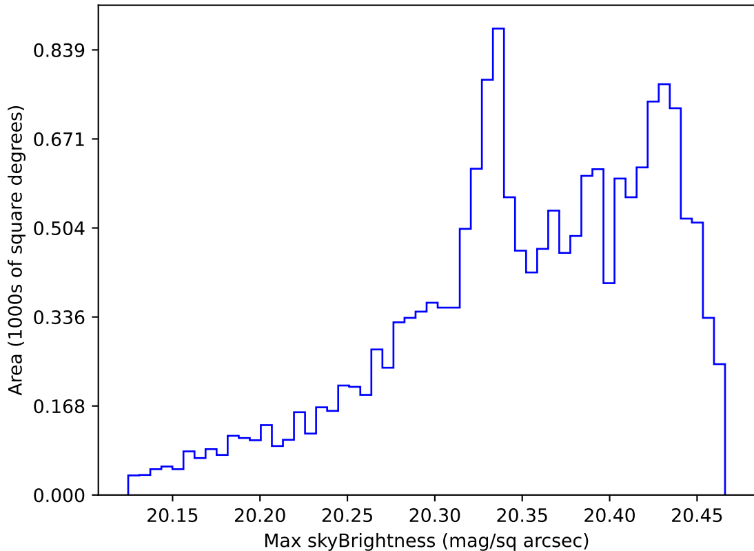
roll_pause_mjdp120_v3.4_10yrs WFD i band: Max skyBrightness
