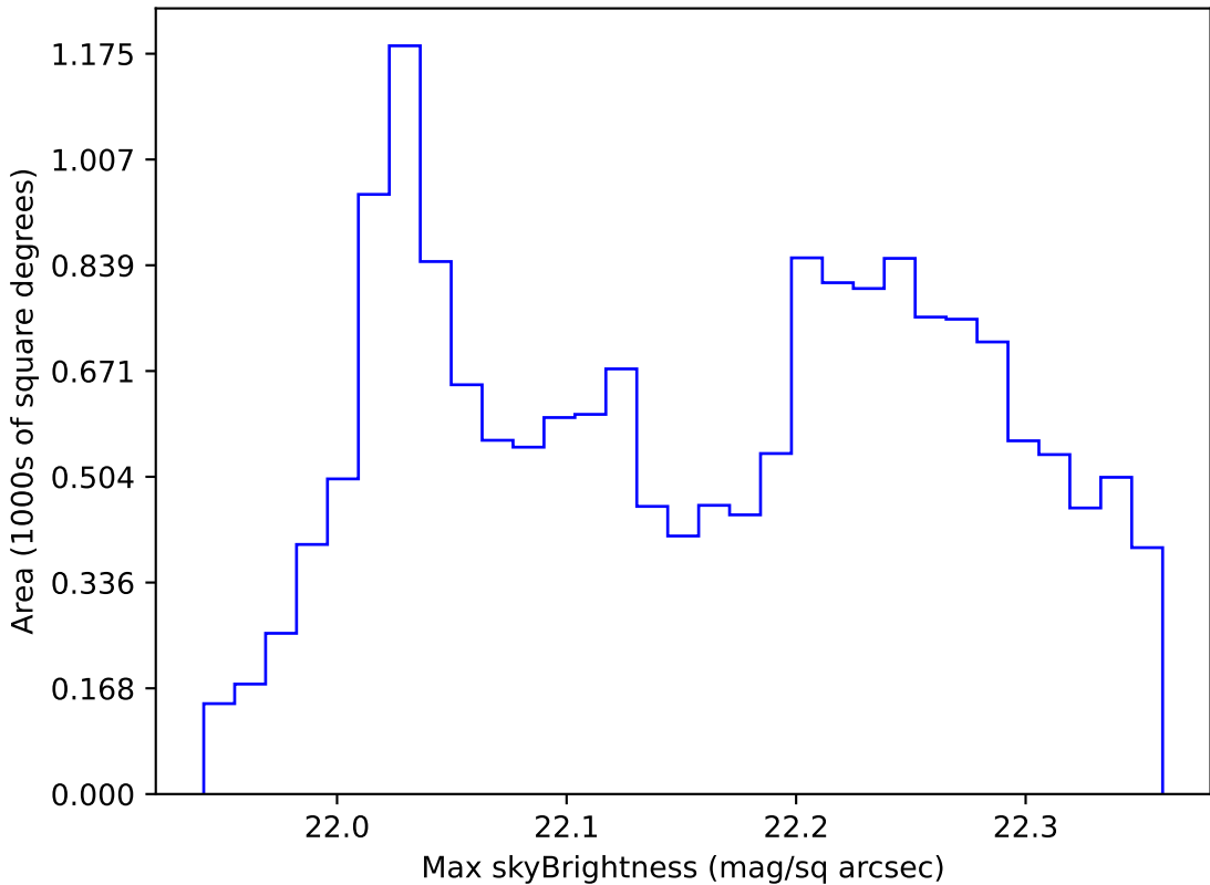
roll_pause_mjdp120_v3.4_10yrs WFD g band: Max skyBrightness
