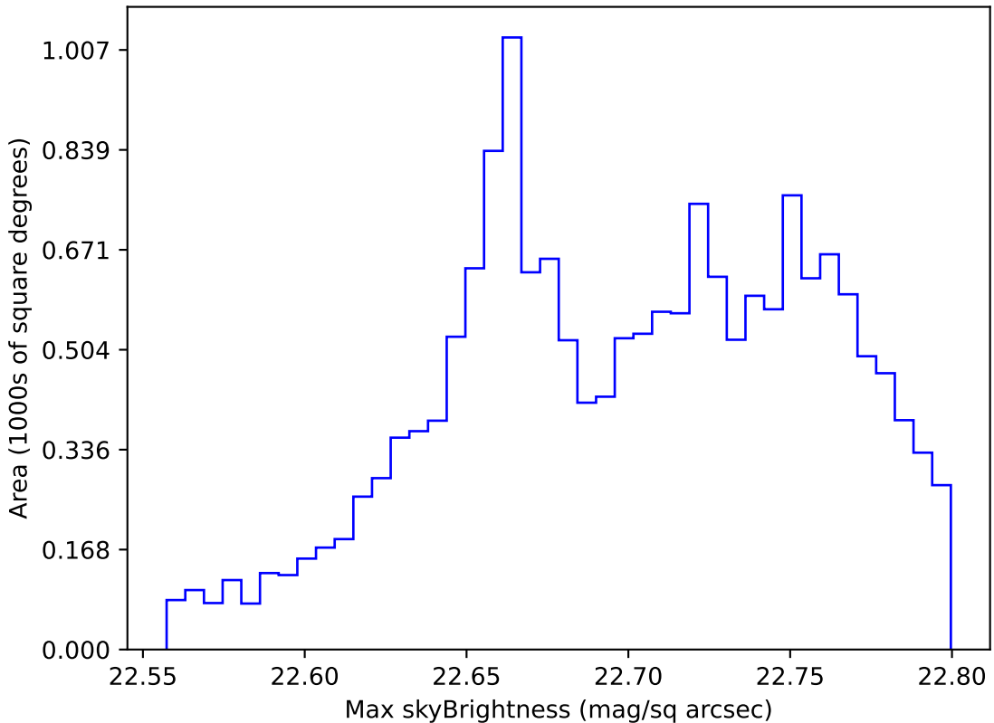
roll_pause_mjdp120_v3.4_10yrs WFD all bands: Max skyBrightness
