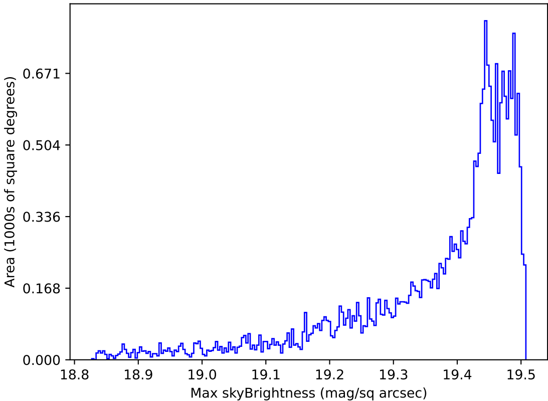
roll_pause_mjdp120_v3.4_10yrs All sky z band: Max skyBrightness
