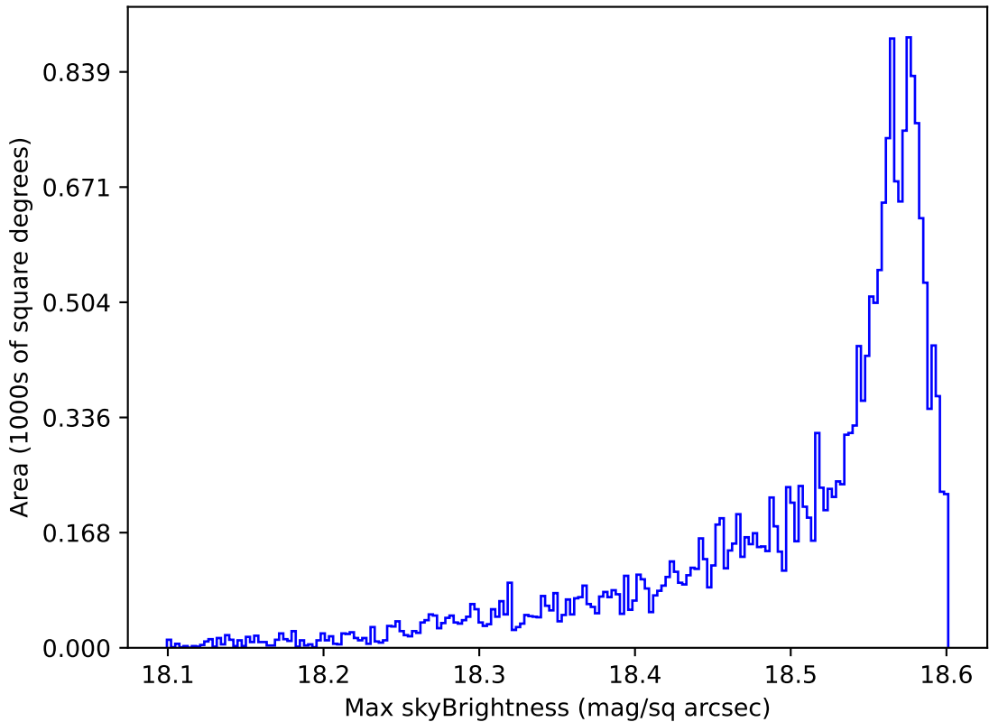
roll_pause_mjdp120_v3.4_10yrs All sky y band: Max skyBrightness
