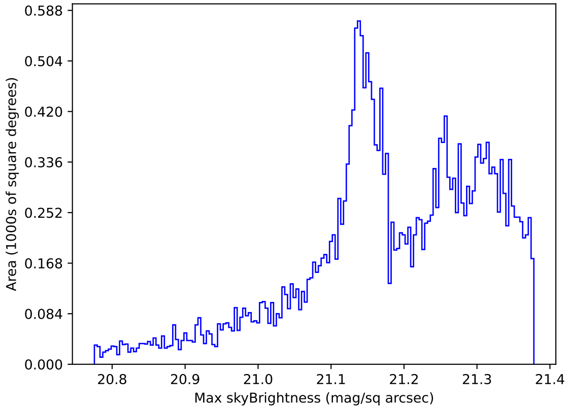
roll_pause_mjdp120_v3.4_10yrs All sky r band: Max skyBrightness
