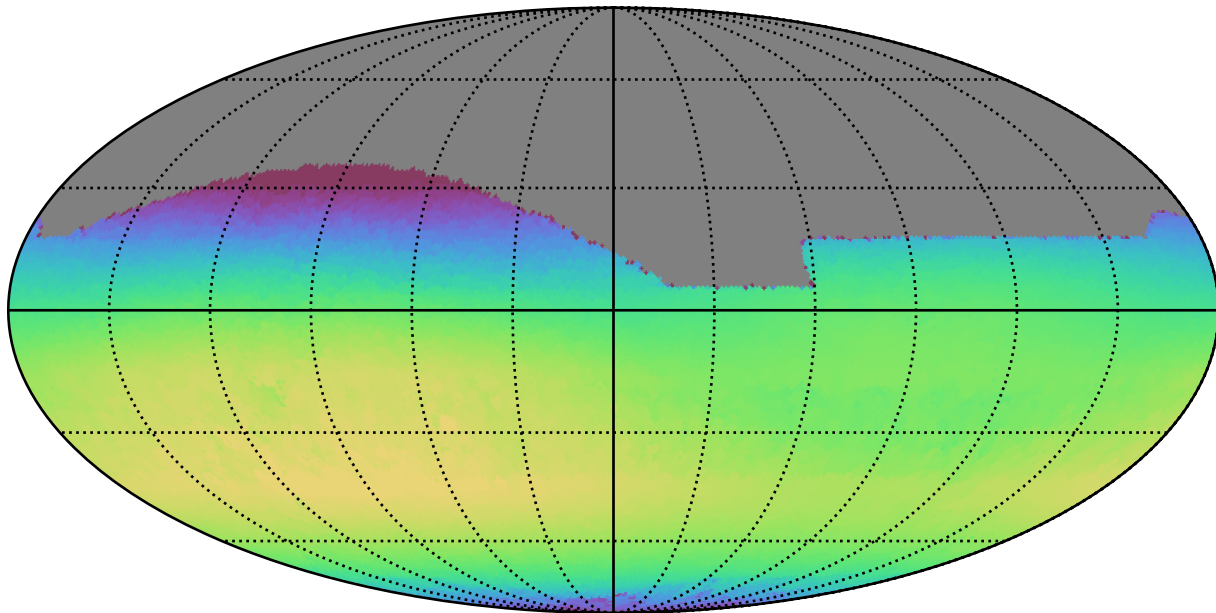
roll_pause_mjdp120_v3.4_10yrs All sky i band: Max skyBrightness
