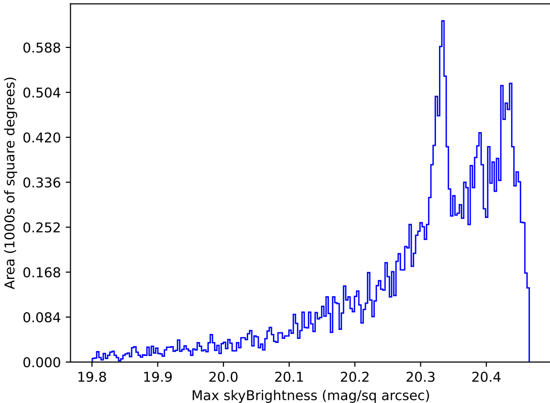
roll_pause_mjdp120_v3.4_10yrs All sky i band: Max skyBrightness
