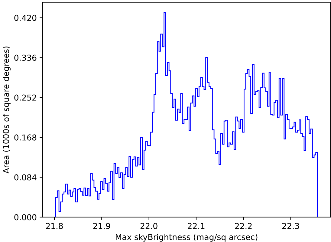
roll_pause_mjdp120_v3.4_10yrs All sky g band: Max skyBrightness
