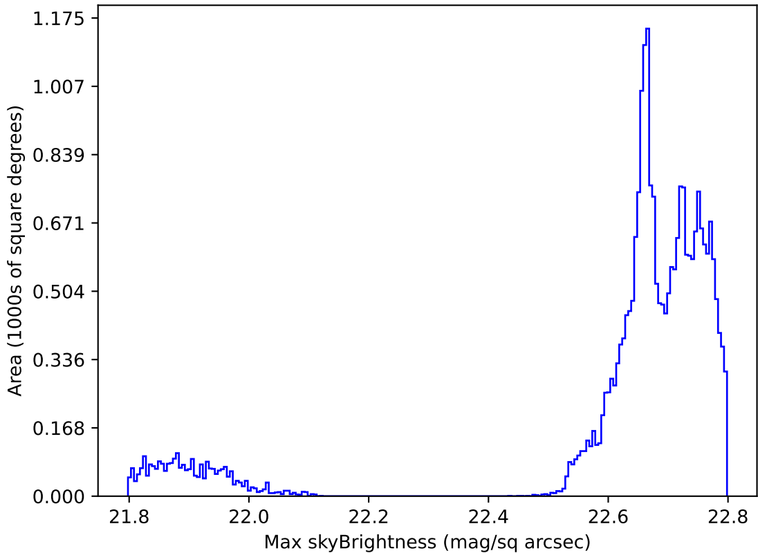
roll_pause_mjdp120_v3.4_10yrs All sky all bands: Max skyBrightness
