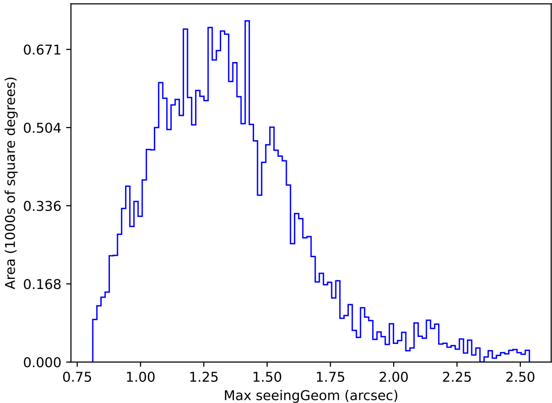
roll_pause_mjdp120_v3.4_10yrs Yr 1 z band: Max seeingGeom
