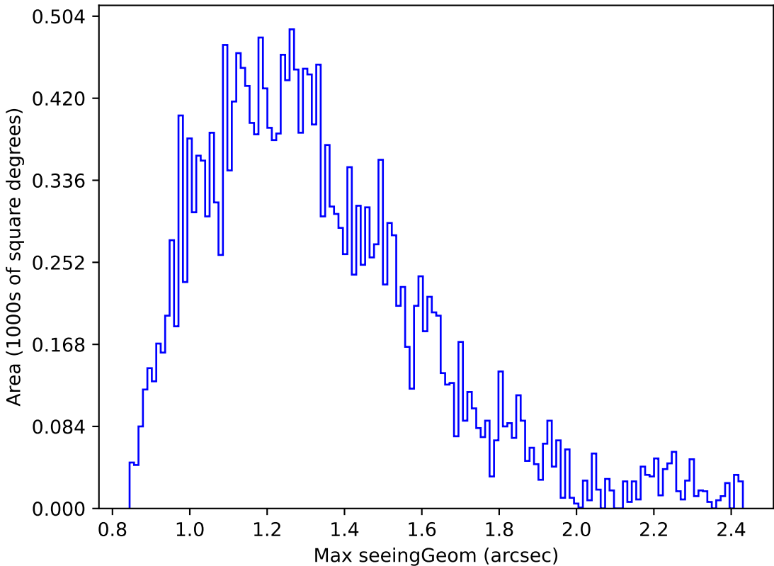
roll_pause_mjdp120_v3.4_10yrs Yr 1 y band: Max seeingGeom
