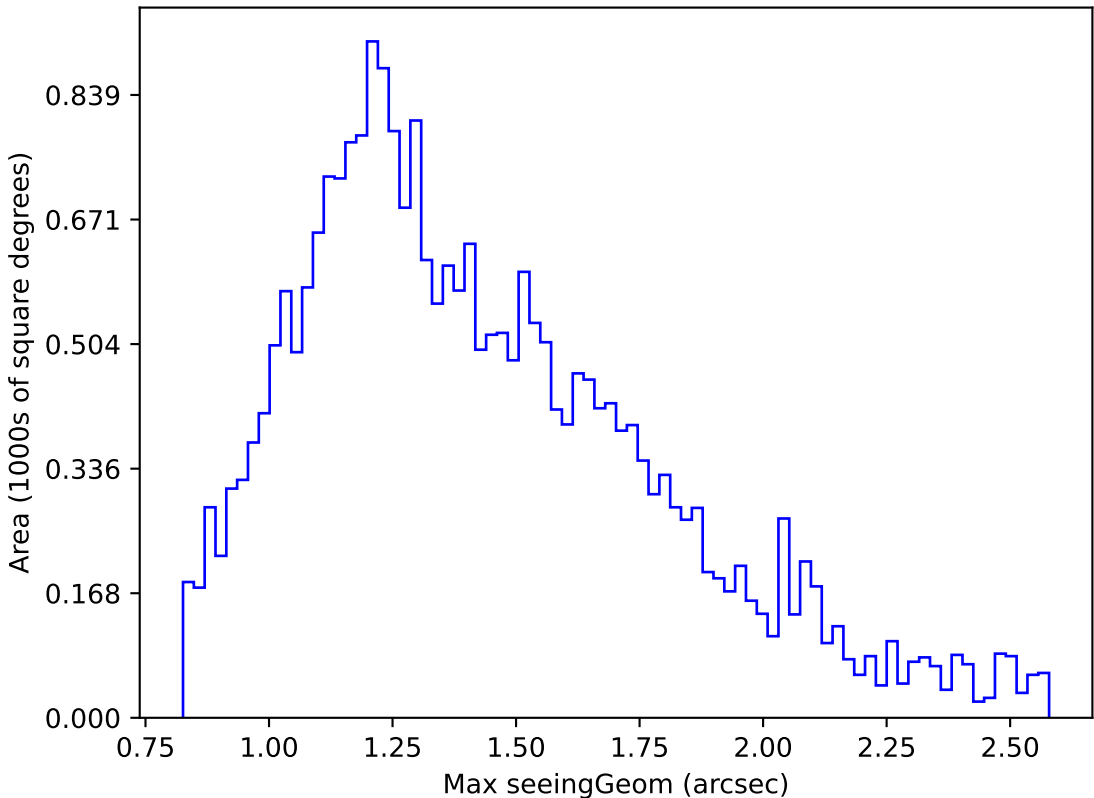
roll_pause_mjdp120_v3.4_10yrs Yr 1 i band: Max seeingGeom
