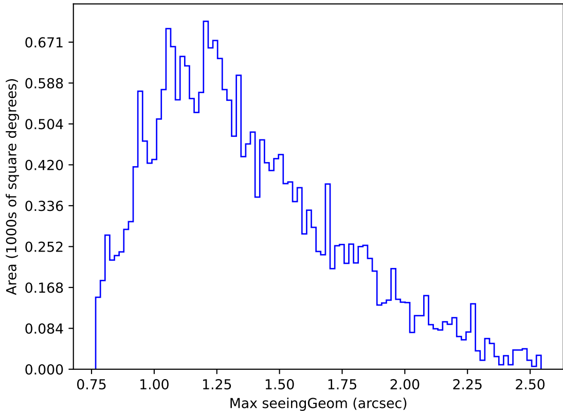
roll_pause_mjdp120_v3.4_10yrs Yr 1 g band: Max seeingGeom
