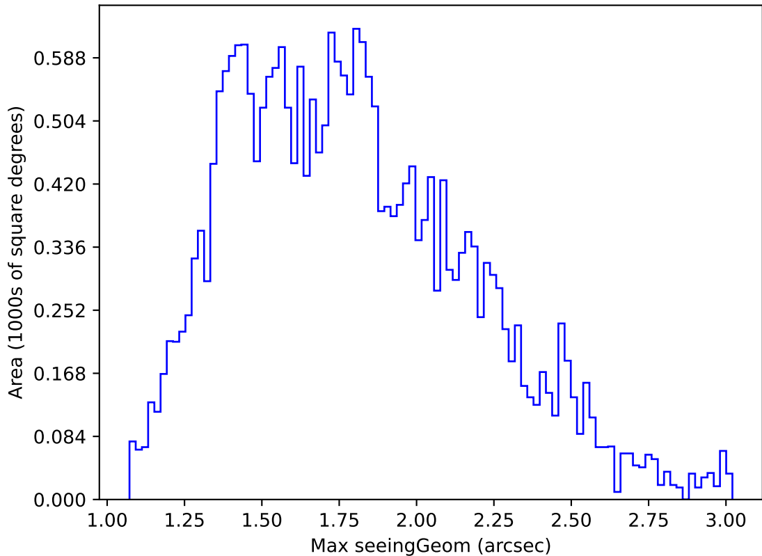
roll_pause_mjdp120_v3.4_10yrs Yr 1 all bands: Max seeingGeom
