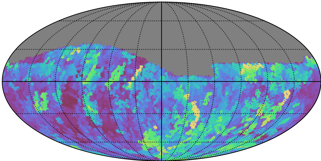
roll_pause_mjdp120_v3.4_10yrs Yr 1 r band: Max seeingEff
