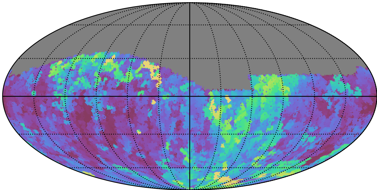
roll_pause_mjdp120_v3.4_10yrs Yr 1 g band: Max seeingEff
