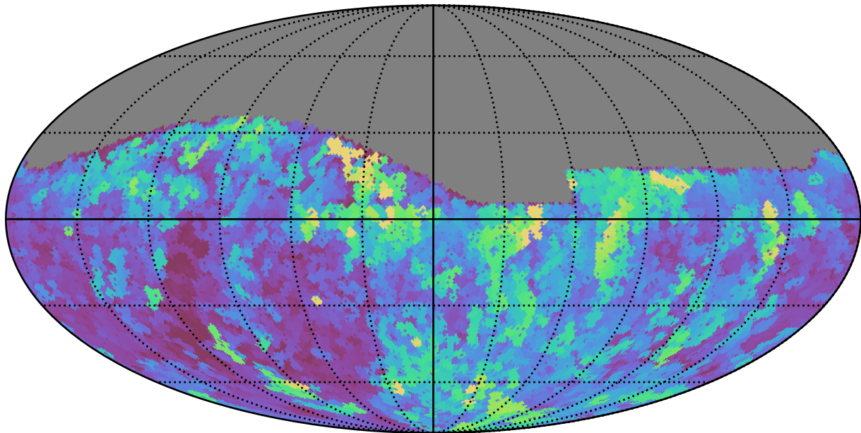
roll_pause_mjdp120_v3.4_10yrs Yr 1 all bands: Max seeingEff
