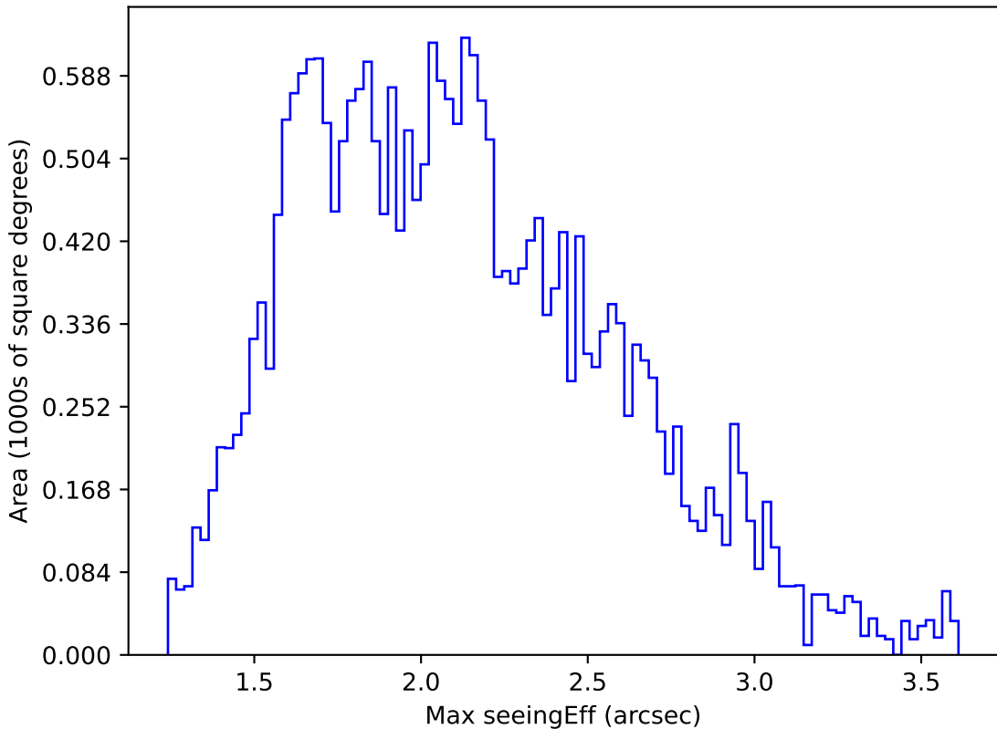
roll_pause_mjdp120_v3.4_10yrs Yr 1 all bands: Max seeingEff
