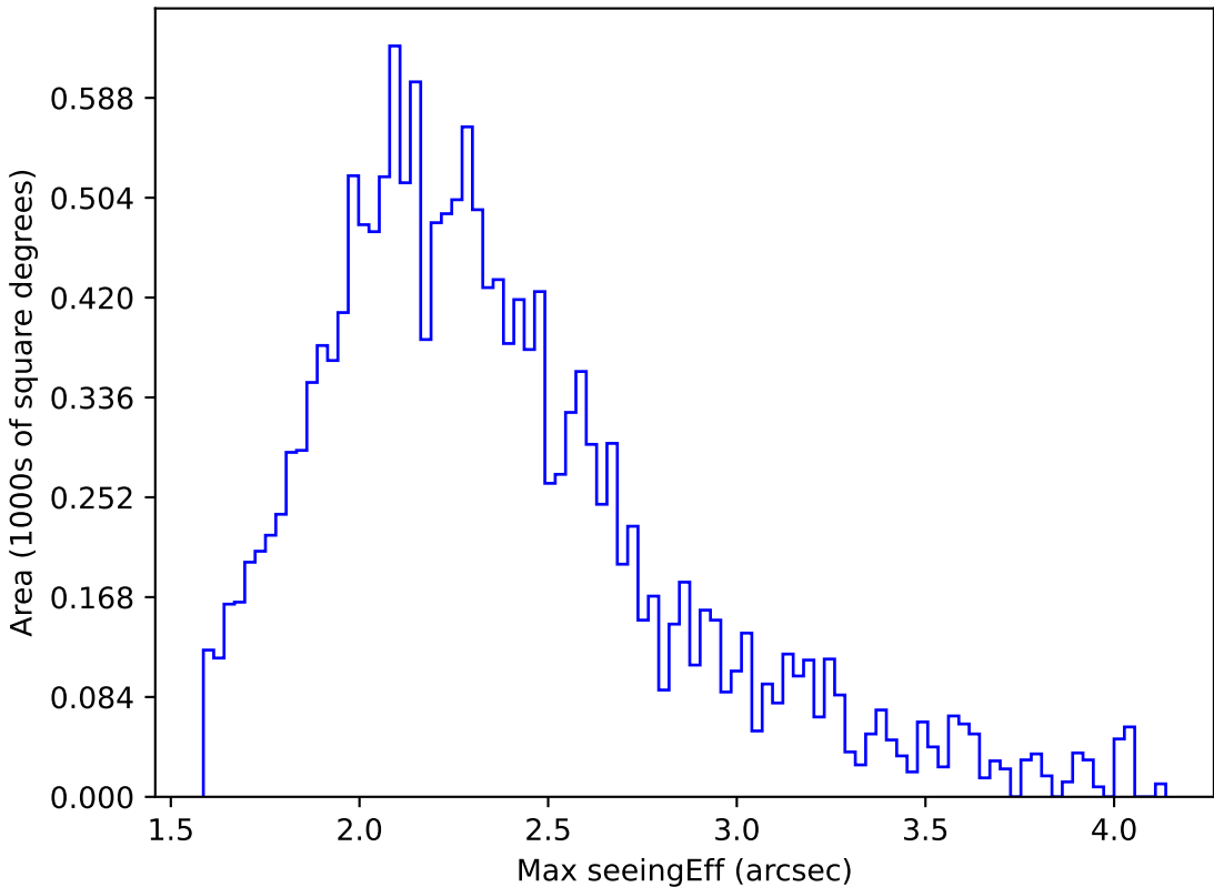
roll_pause_mjdp120_v3.4_10yrs WFD y band: Max seeingEff
