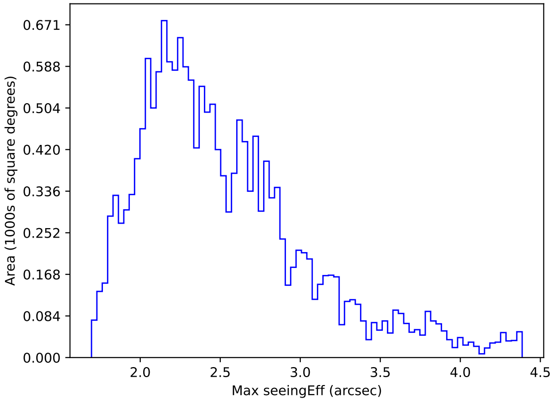
roll_pause_mjdp120_v3.4_10yrs WFD u band: Max seeingEff
