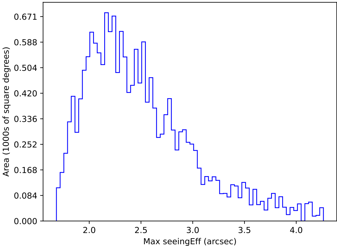
roll_pause_mjdp120_v3.4_10yrs WFD g band: Max seeingEff
