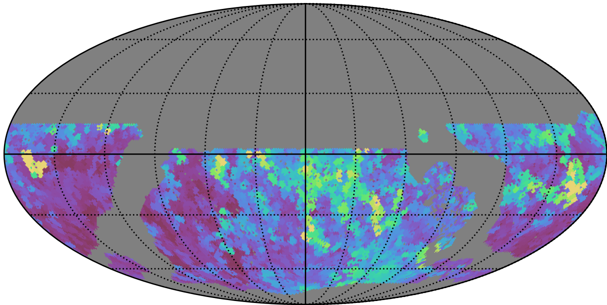
roll_pause_mjdp120_v3.4_10yrs WFD all bands: Max seeingEff
