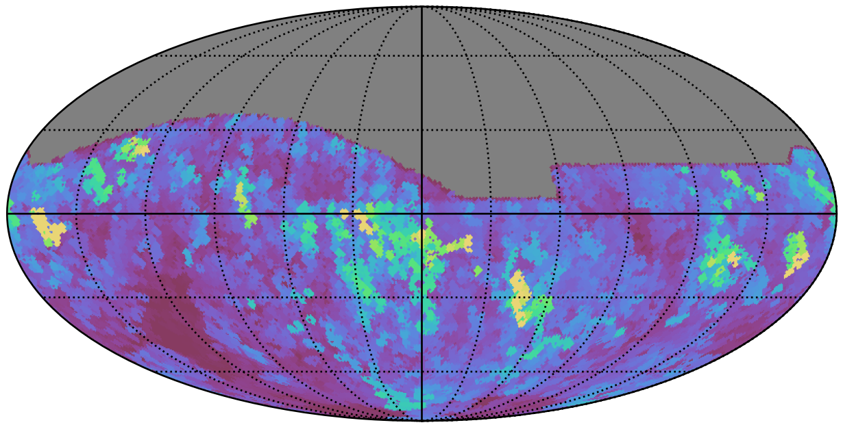
roll_pause_mjdp120_v3.4_10yrs All sky z band: Max seeingEff
