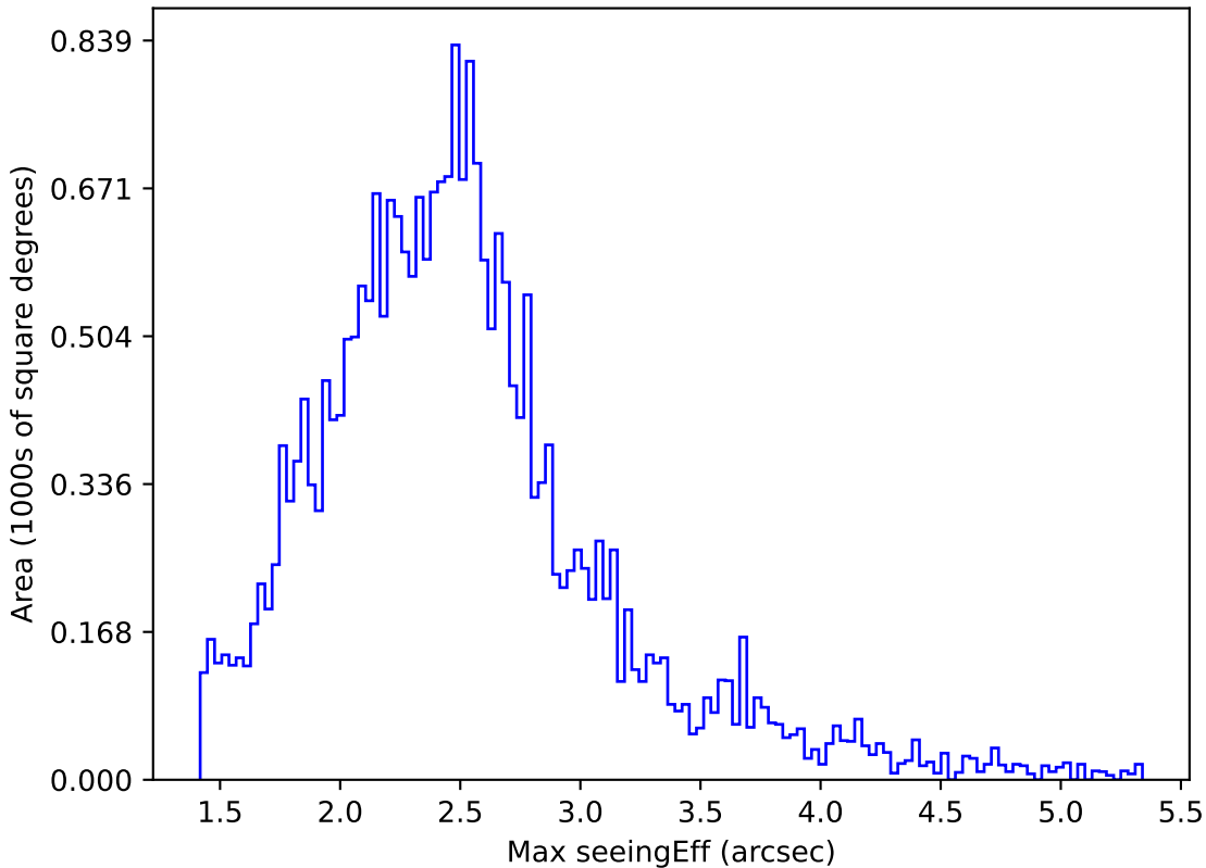
roll_pause_mjdp120_v3.4_10yrs All sky z band: Max seeingEff
