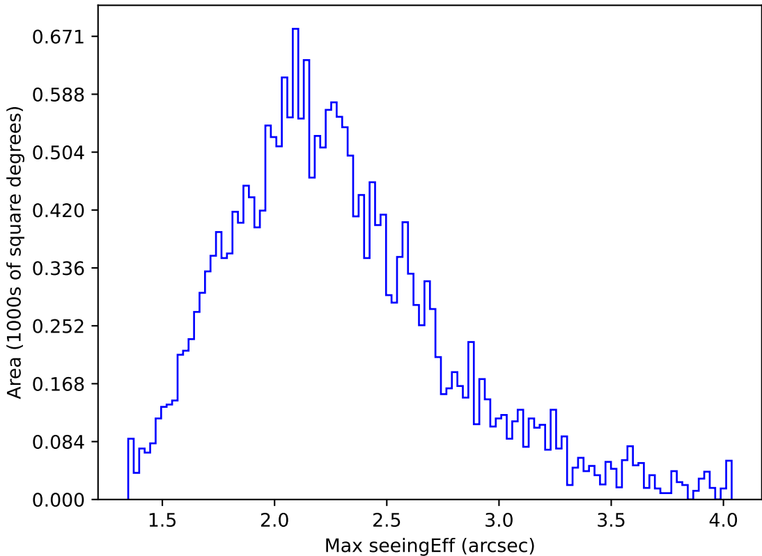
roll_pause_mjdp120_v3.4_10yrs All sky y band: Max seeingEff
