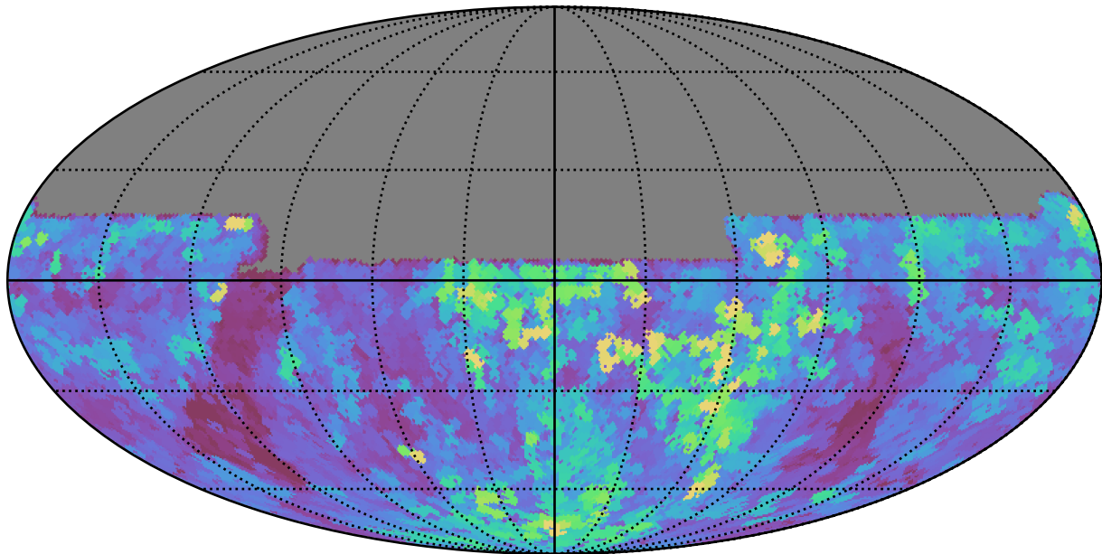
roll_pause_mjdp120_v3.4_10yrs All sky u band: Max seeingEff
