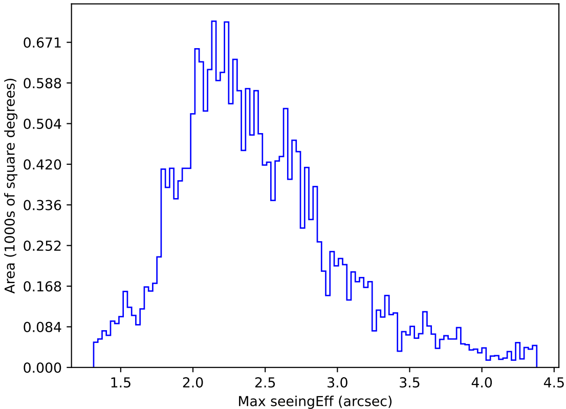
roll_pause_mjdp120_v3.4_10yrs All sky u band: Max seeingEff
