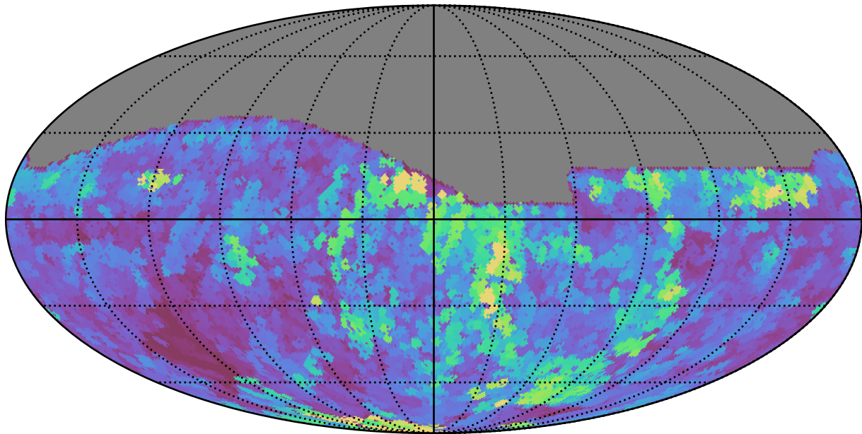
roll_pause_mjdp120_v3.4_10yrs All sky r band: Max seeingEff
