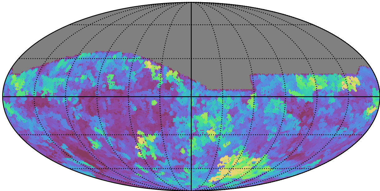
roll_pause_mjdp120_v3.4_10yrs All sky g band: Max seeingEff
