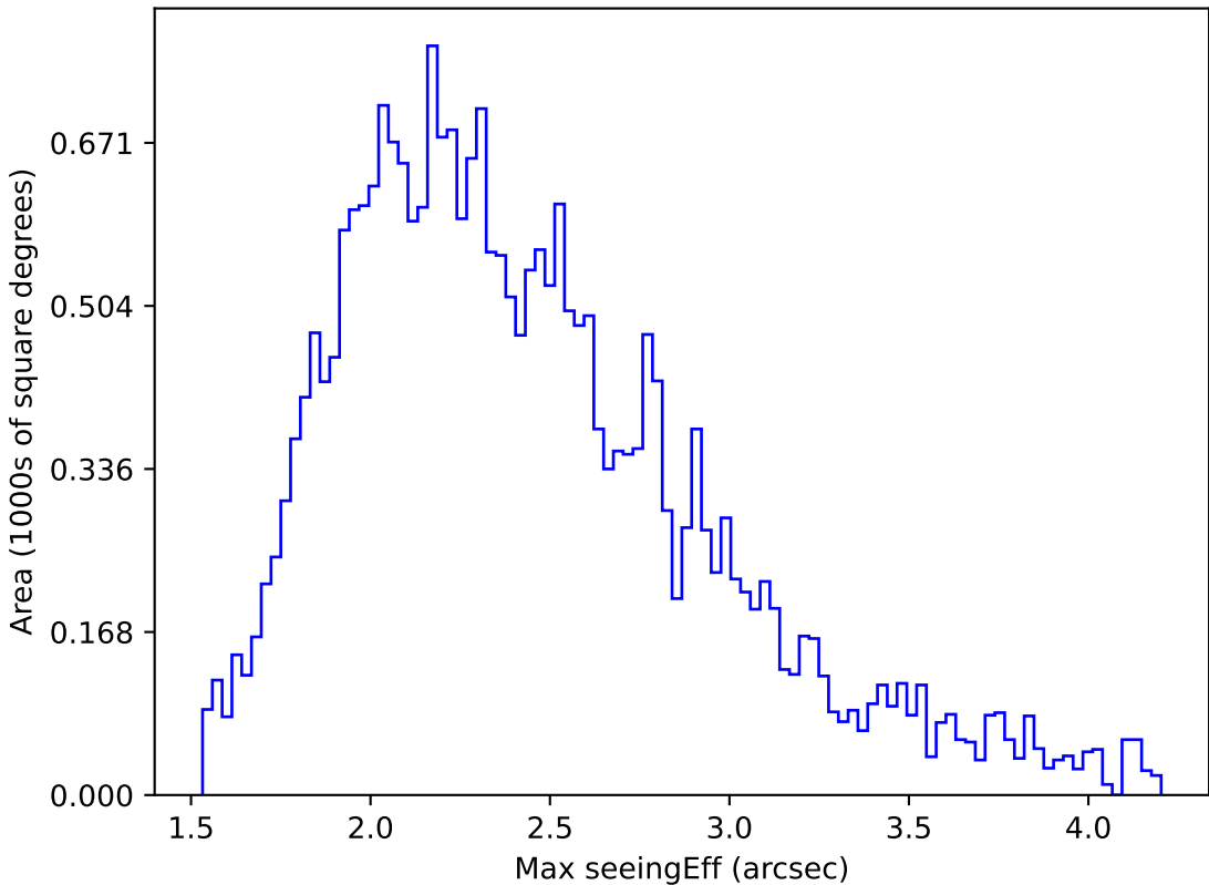
roll_pause_mjdp120_v3.4_10yrs All sky g band: Max seeingEff
